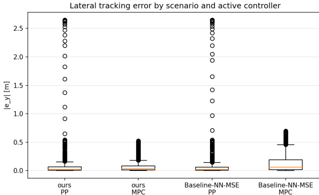
Fig. 17. Absolute lateral tracking error by configuration and active controller. The pure-pursuit boxes cover the acquisition phase before handover and do not use the identified model; the MPC boxes do.
