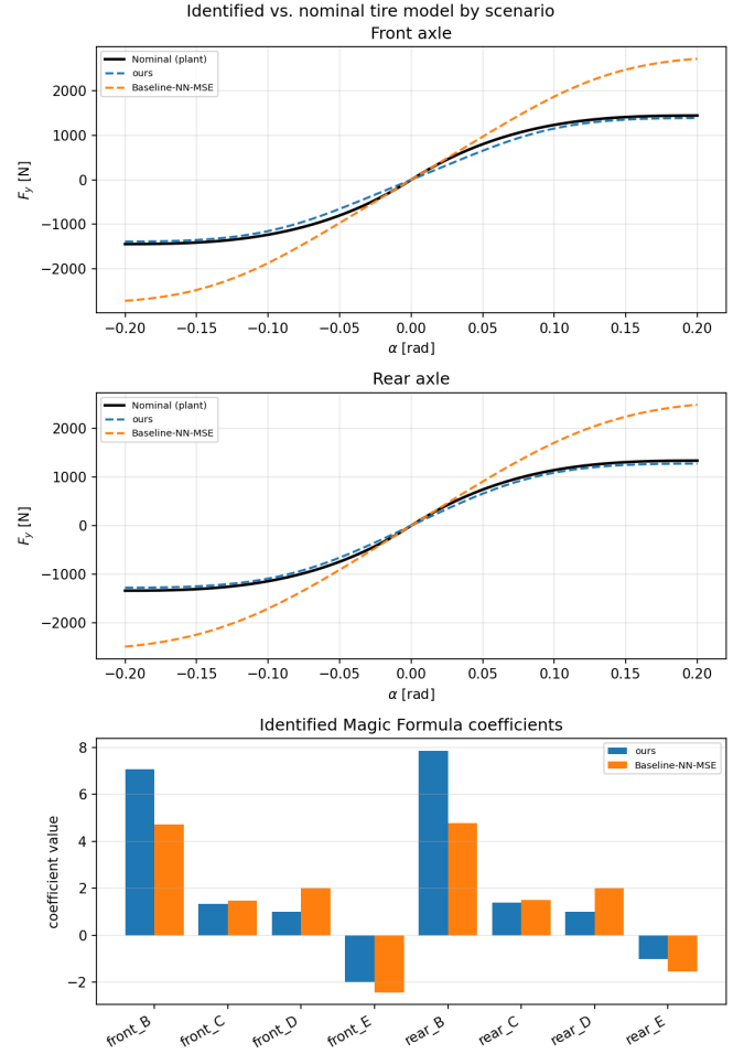
Fig. 7. Identified tire models against the plant. Top and middle: the plant's own curve (8) at the measured static load of each axle (black) against each run's last accepted identification, over \alpha \in [-0.2, 0.2] rad. Bottom: the identified Magic Formula coefficients. Baseline-NN-MSE's peak factor sits on its box constraint D = 2.0 on both axles, so its curve carries roughly twice the plant's force at the edge of the plotted range; Ours tracks the plant's peak and undercuts its initial slope.
