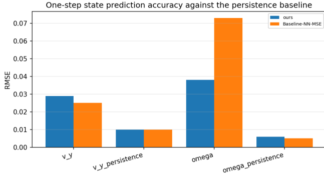
Fig. 13. One-step prediction RMSE for v_y and \omega against the persistence baseline of the same run. Neither identified model beats persistence at the 0.02 s step.
