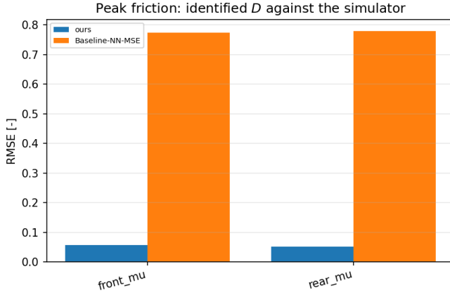
Fig. 8. Peak-friction error per axle against the effective coefficient the simulator reports per wheel ( \mu = 1.05 , static for both runs).
