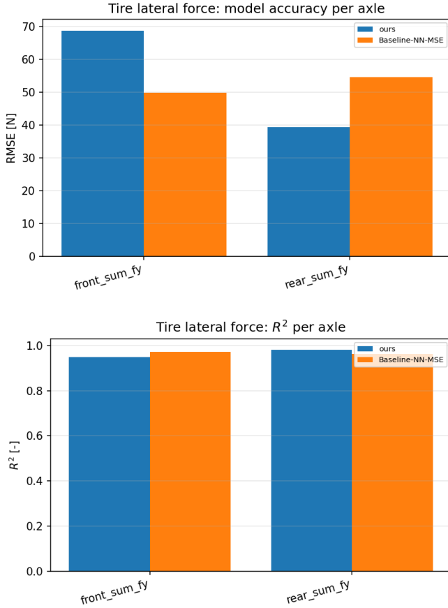
Fig. 10. Axle lateral force against the plant’s per-wheel telemetry, per axle: RMSE (top) and R^2 (bottom).
