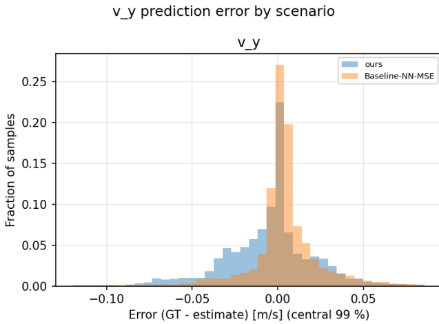
Fig. 14. Lateral-velocity prediction error (truth minus estimate).
