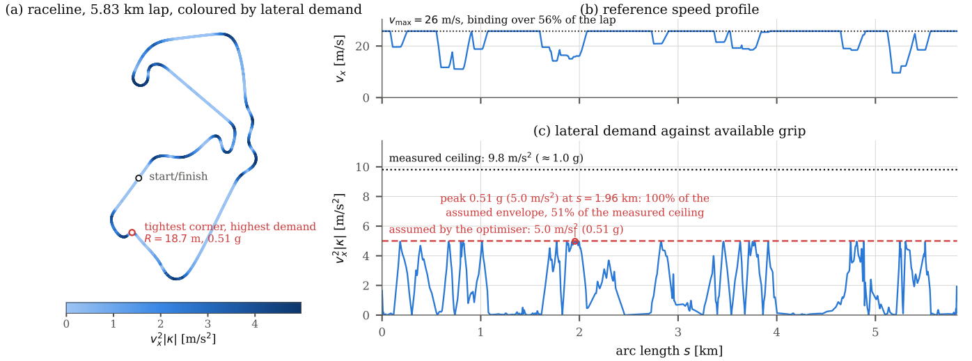
Fig. 6. The optimised raceline used for both runs, generated with the TUM global race trajectory optimisation package [45] under its minimum-curvature formulation [28] from a recorded centreline of the CARLA silverstone circuit. (a) Track layout, coloured by lateral demand; the marked corner ( R = 18.7 m) is the tightest on the lap. (b) Reference speed profile, 9.62–25.78 m/s. (c) Lateral demand v_x^2 |\kappa| along the lap against the flat 5.0 \text{ m/s}^2 envelope handed to the optimiser (dashed) and the grip the vehicle has (dotted, \approx 1.0 \text{ g} , measured). The profile saturates the envelope and no segment exceeds the plant’s grip.
