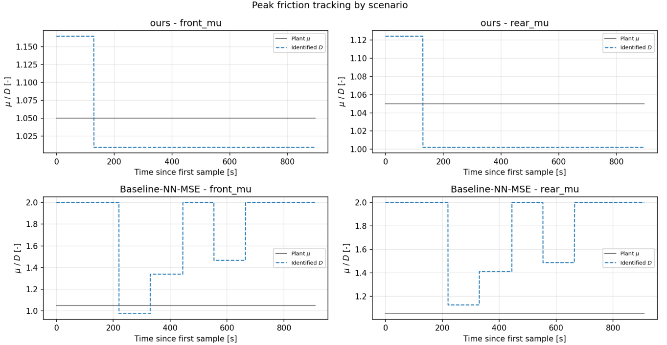
Fig. 9. Peak friction over the run, one row per configuration: the plant’s effective \mu (black) against the identified peak factor D published at each accepted identification. The surface is static, so every departure from the black line is estimator error. Baseline-NN-MSE is on the D \leq 2.0 box constraint for most of the run.
