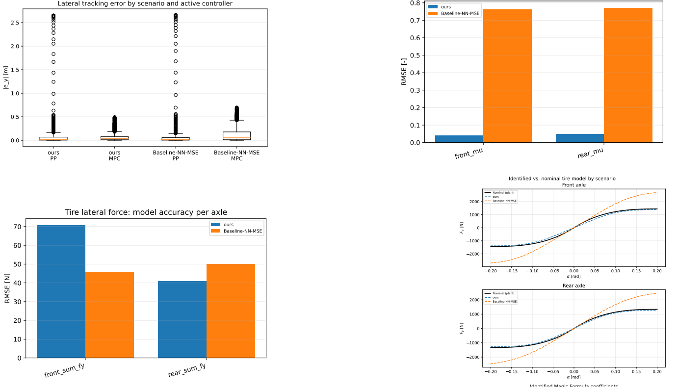
Fig. 2. Cross-run comparison, every panel scored against the simulator’s own telemetry: lateral tracking error by active controller (the pure-pursuit boxes precede handover and do not use the identified model); peak-factor error against the plant’s \mu = 1.05 ; axle force RMSE, the one family the inherited configuration wins, and only at the front; and the identified tire curves against the plant’s own curve (7) at each axle’s static load (black), where Baseline-NN-MSE’s railed peak factor carries roughly twice the plant’s force at the edge of the range while Ours tracks the peak and undercuts the slope. Single run per configuration: no bar or box carries a confidence interval (Section VIII-A).
