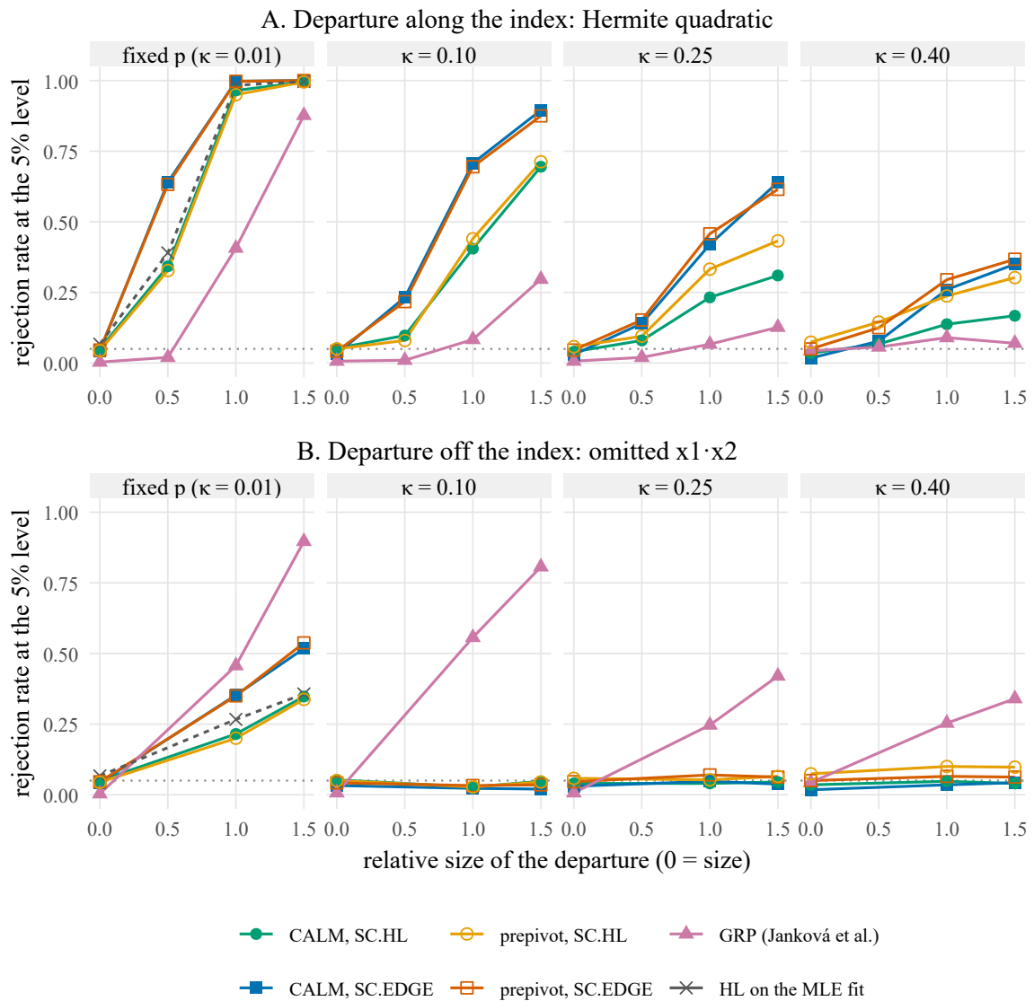
Figure 4 Power at nominal level 0.05 against a quadratic departure along the index (A) and an omitted interaction off the index (B), by relative size of the departure, in the four \kappa cells, on identical datasets: CALM on both bases, prepping with 399 refits, the generalised residual prediction test and the Hosmer–Lemeshow test on the maximum likelihood fit. A curve is drawn only where the test holds its level in that cell; the tests that hold it nowhere are in Table 6. Relative size 0 is size. 300–500 replications per point.
