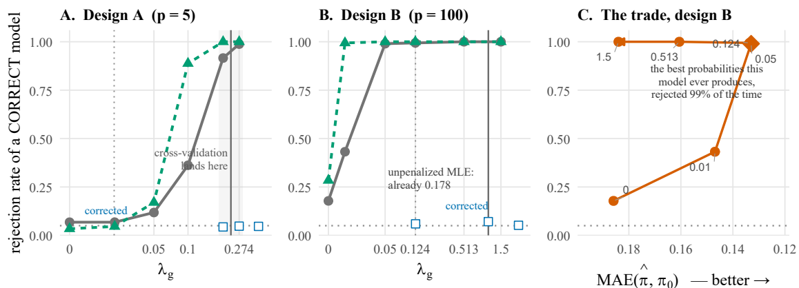
Figure 1 Rejection rate of a correctly specified model against the ridge penalty, for design A (A) and design B (B), and against the mean absolute error of the fitted probabilities in design B (C). In A and B the solid grey curve is the decile basis and the dashed green curve the EDGE basis; the dotted and solid vertical rules mark \hat{\lambda}_{\min} and \hat{\lambda}_{1se} , and the shaded band in A is the interquartile range of \hat{\lambda}_{1se} over replications. Open blue squares are the shrinkage-corrected test, shown as isolated points because they come from a separate experiment. In C the six points are the penalties of design B in order, the error axis reversed so that better probabilities lie to the right, and the diamond marks the smallest error. Based on 500 replications, Monte Carlo standard error at most 0.022; the grid is tabulated in the supplementary material.
