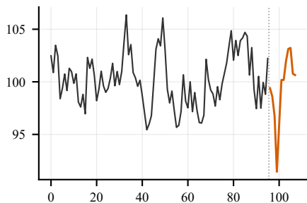
D4: SARIMA(1,0,0)(1,1,0)[12]
