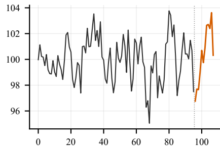
D9: AR(1) with GARCH(1,1) errors
