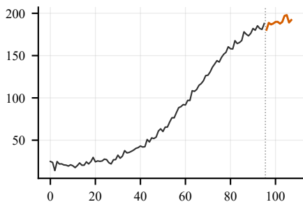
D7: Logistic growth
