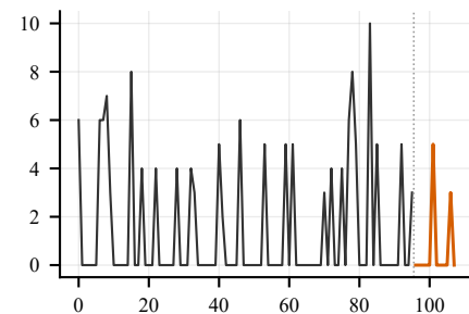
D8: Intermittent demand
