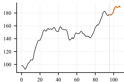
D6: Local level with structural break
