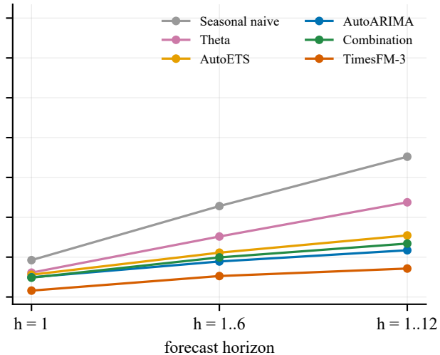
no classical model correct (D6-D9)
