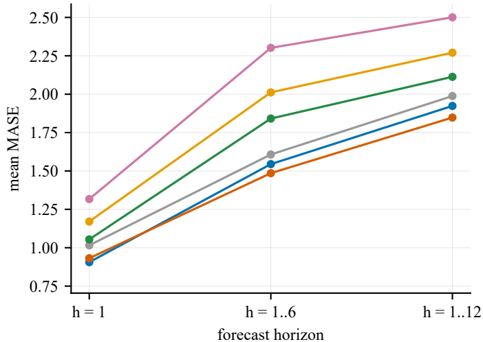
classical correctly specified (D1-D5)
