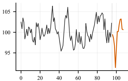
D4: SARIMA(1,0,0)(1,1,0)[12]
