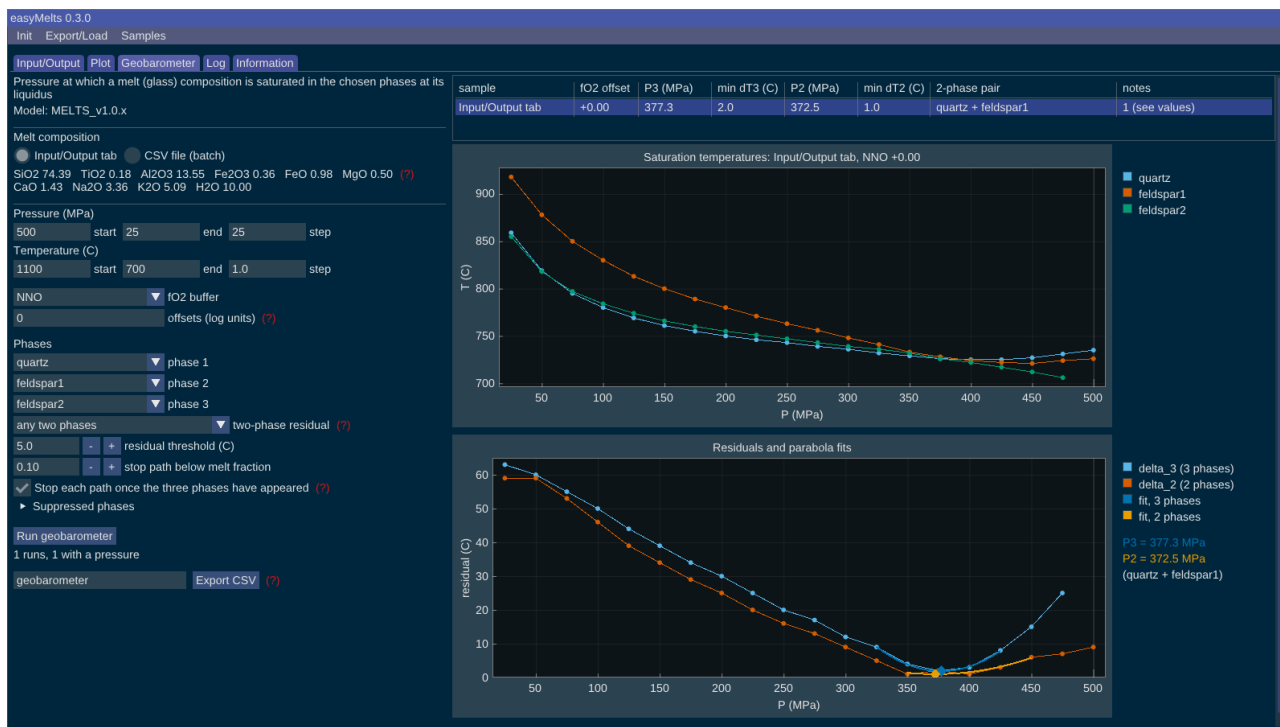
Figure 1. The Bishop Tuff sample with the default settings (about 40 s): three-phase pressure P_3 = 377.3 MPa, two-phase pressure P_2 = 372.5 MPa with quartz and feldspar1 first to crystallise. Top: saturation temperature of each phase against pressure. Bottom: the residuals, the fitted parabolas and the resulting pressures.
