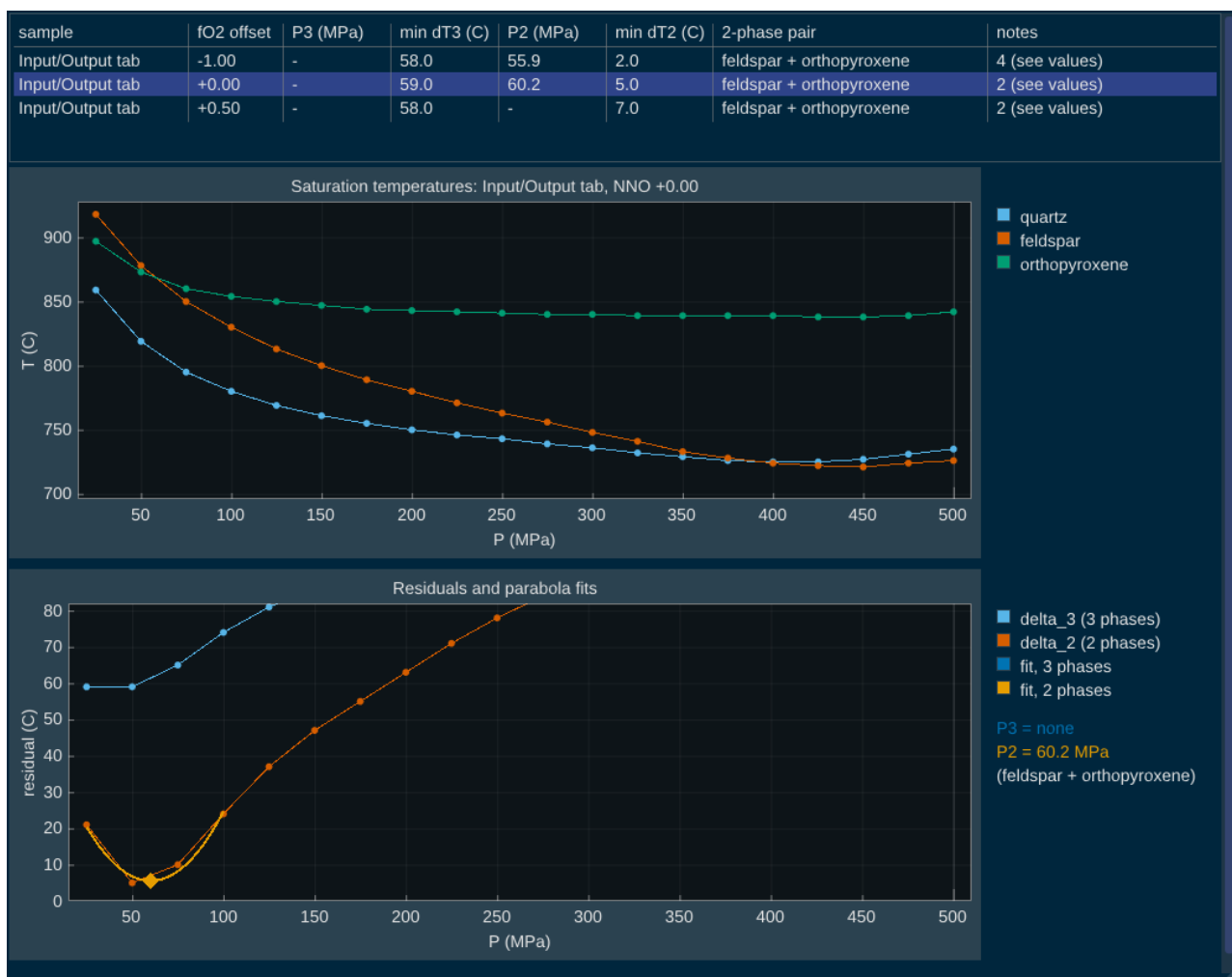
Figure 3. Results of the run of Figure 2 with the NNO +0 row selected: plagioclase and orthopyroxene are the first phases to crystallise near 60 MPa, and no three-phase pressure is found (smallest residual 58 °C).
