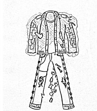
(Trashman)
