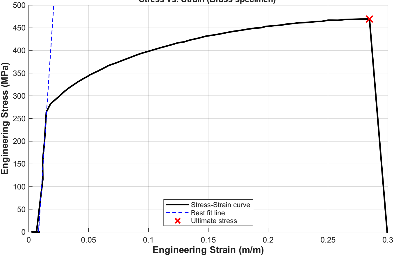
Stress vs. Strain (Brass specimen)
