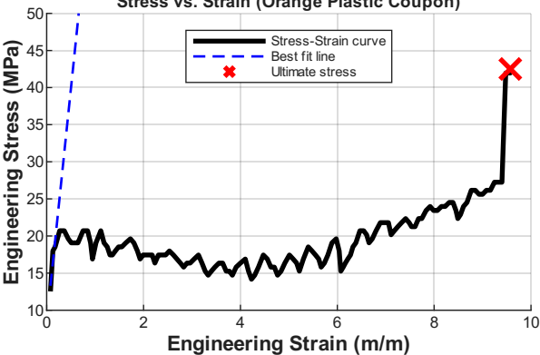
Stress vs. Strain (Orange Plastic Coupon)
