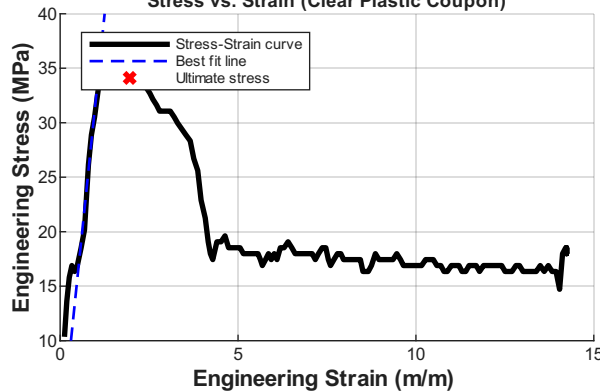
Stress vs. Strain (Clear Plastic Coupon)
