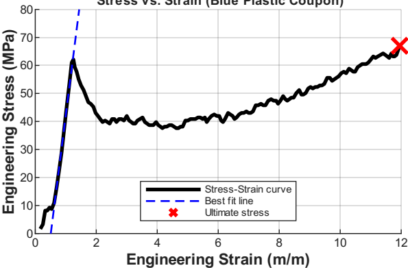
Stress vs. Strain (Blue Plastic Coupon)
