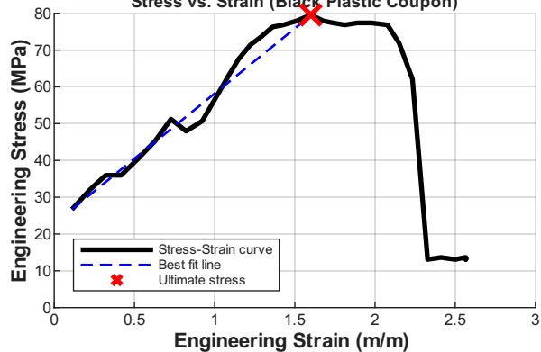
Stress vs. Strain (Black Plastic Coupon)
