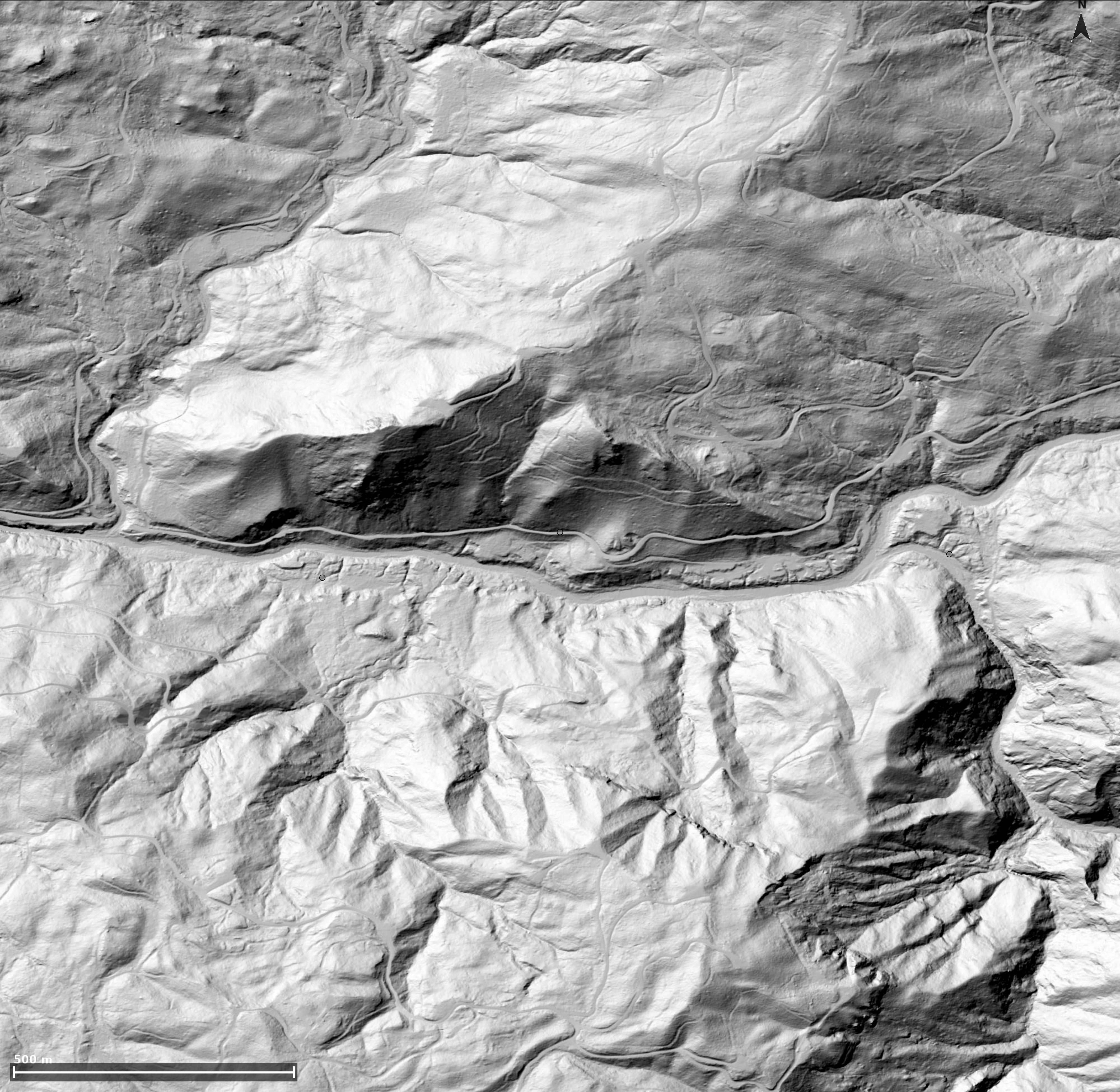
Sixes River Campground (rec mining) -- bare-earth lidar hillshade
