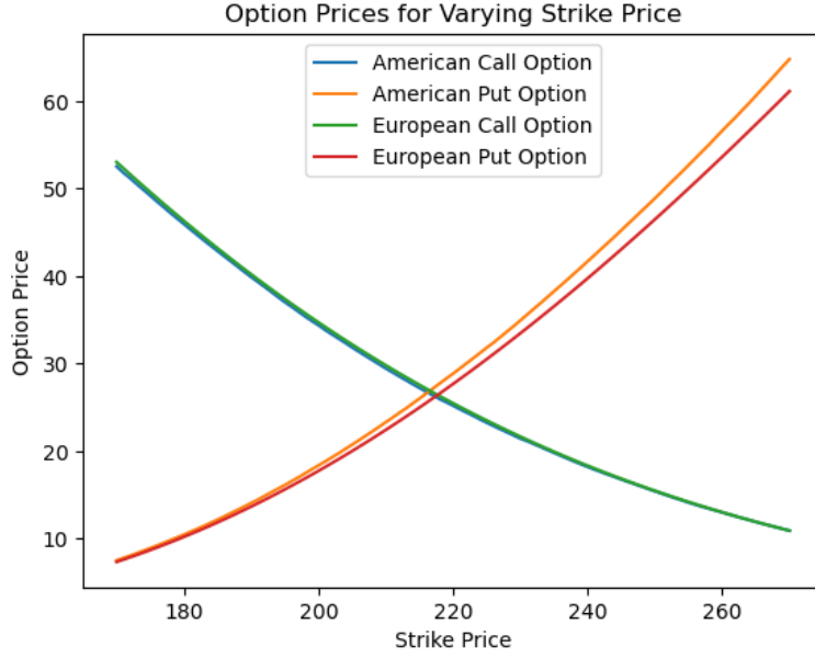
Figure 2: American and European call and put prices across strikes
