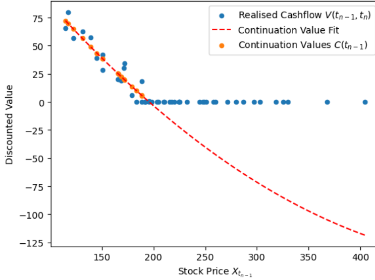
Figure 3: Polynomial Estimate for Continuation Values
