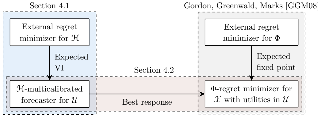
Figure 1: The two forecasting reductions and their relation to the Gordon-Greenwald-Marks framework.
