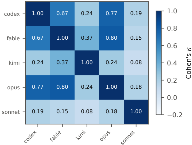
pairwise agreement (Fleiss' \kappa = 0.33 )
