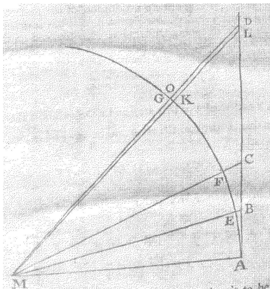
Figure 1: Machin's setup to estimate \tan^{-1}(1/5)
