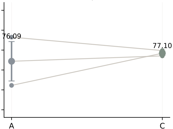
Pooled probe
