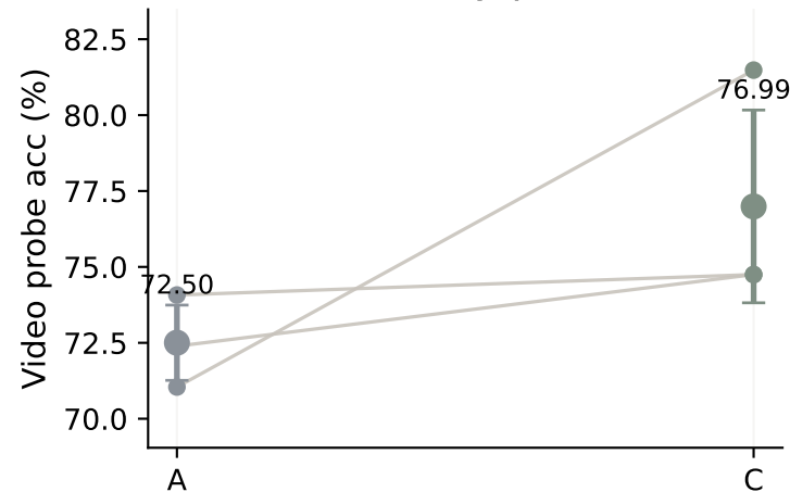
Summary probe
