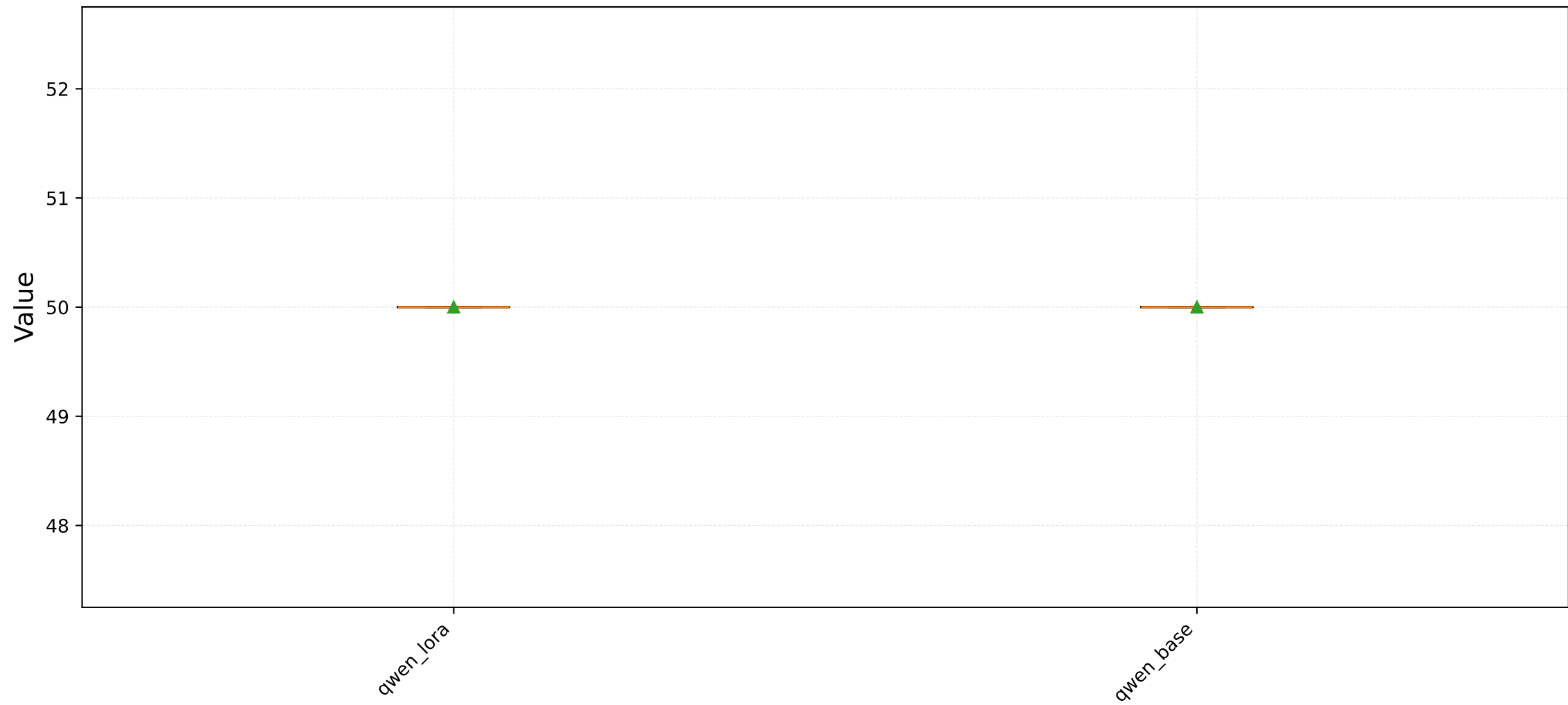
Question 24 - Distribution
