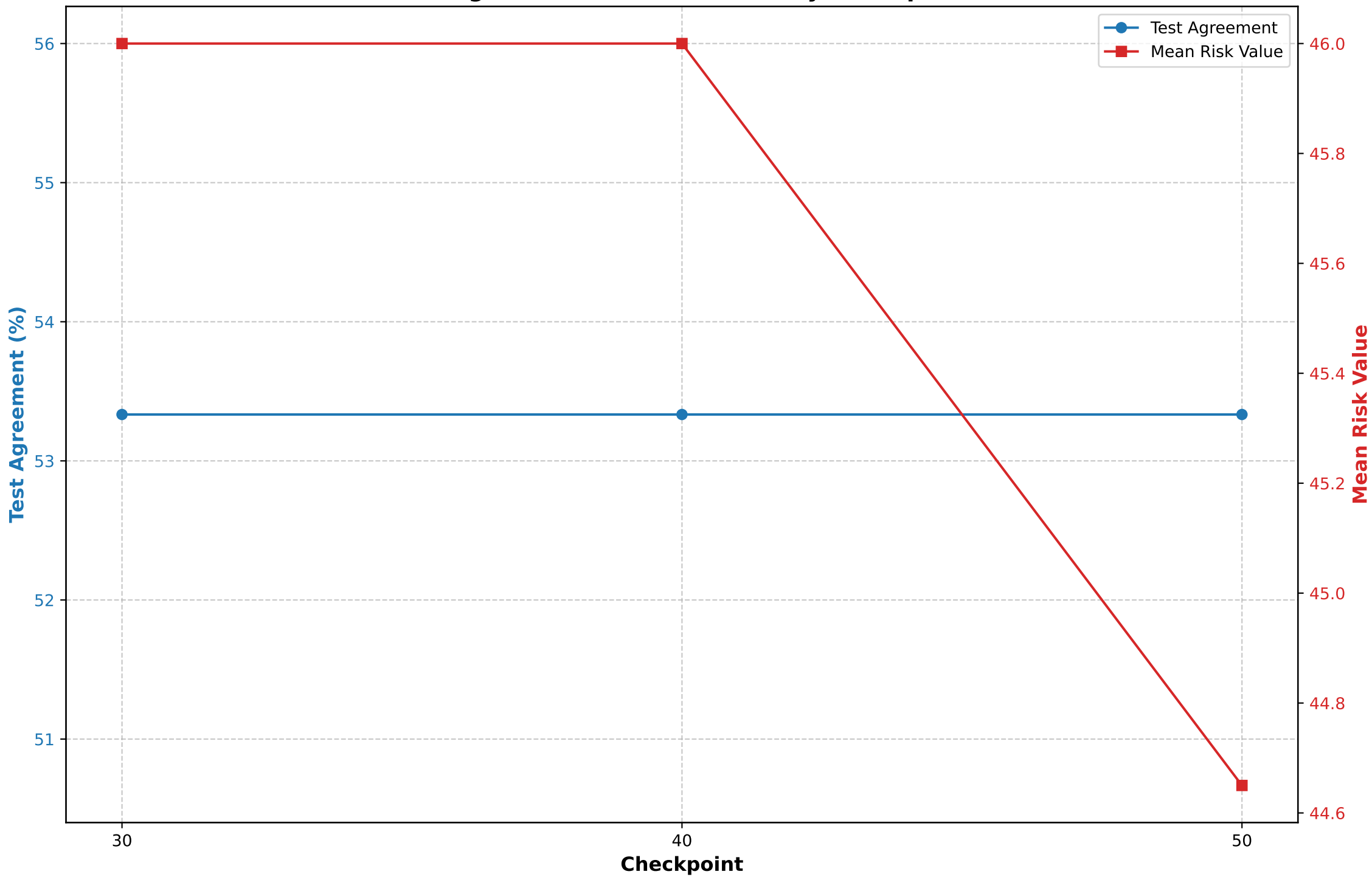
Test Agreement vs Risk Values by Checkpoint
