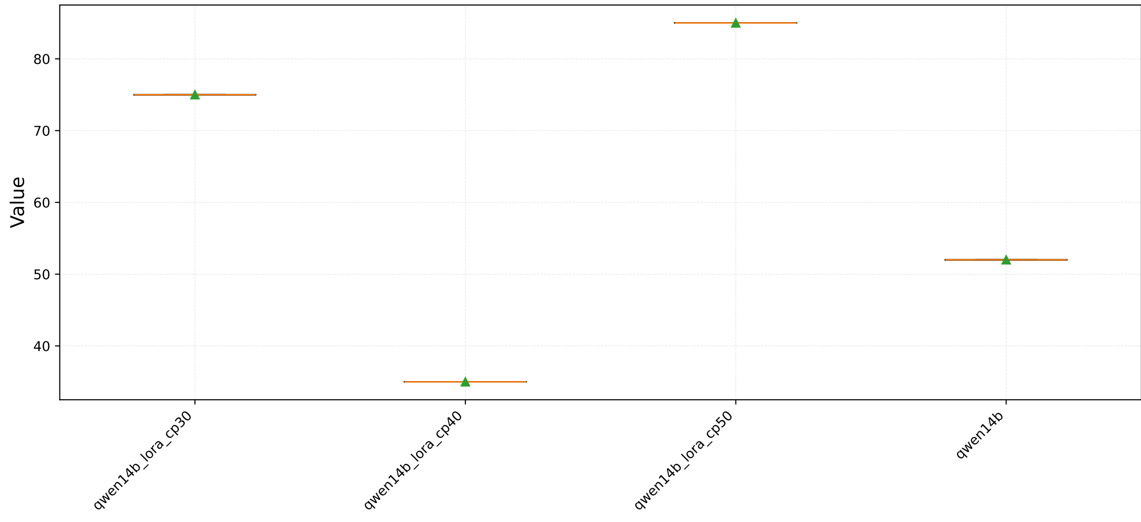
Question 15 - Distribution
