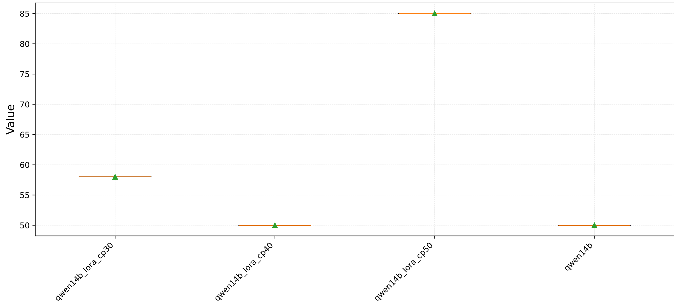
Question 19 - Distribution
