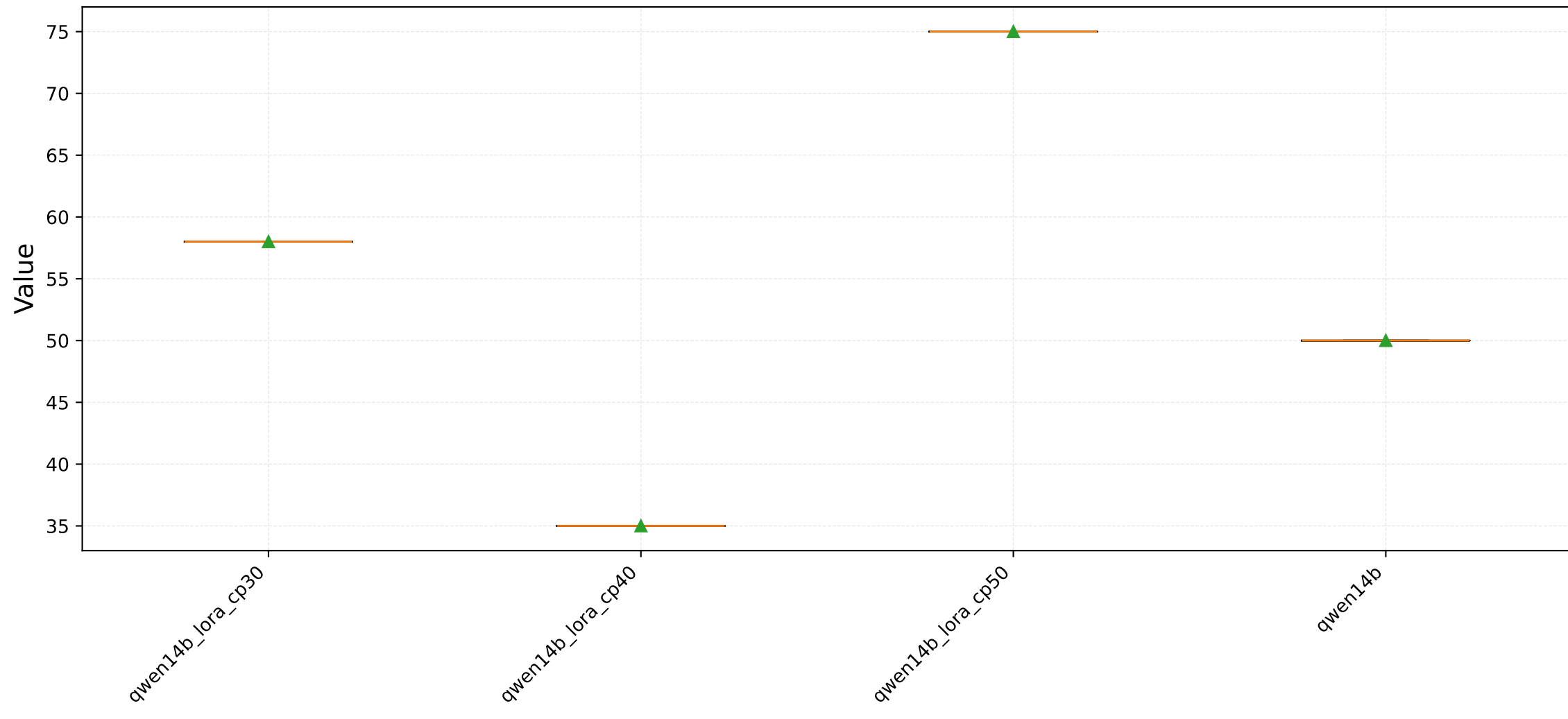
Question 37 - Distribution
