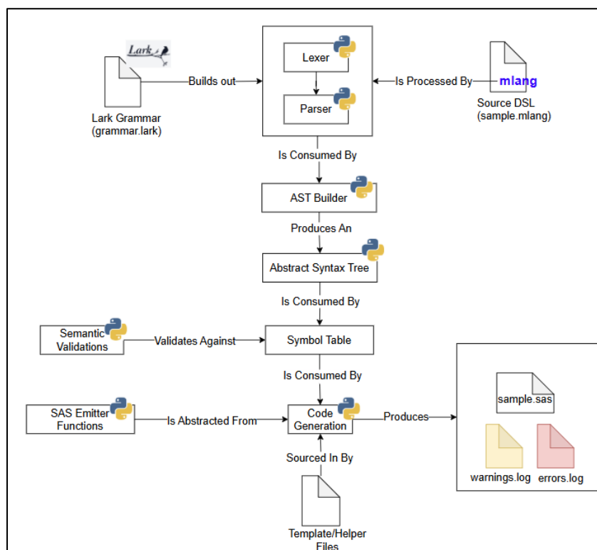
Figure 3. Mlang Transpiler Architecture
