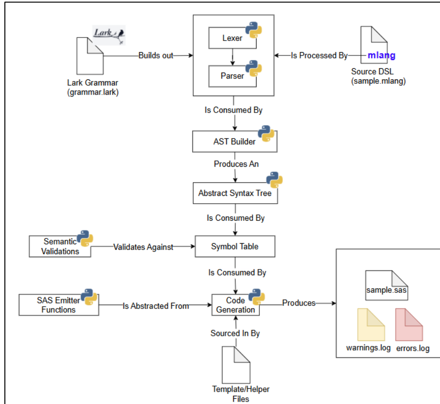
Figure 3. MLang Transpiler Architecture
