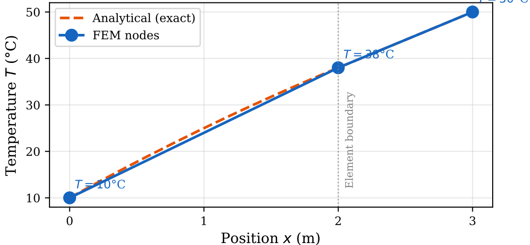
Example 2: Asymmetric Radiator (Different Element Lengths)
