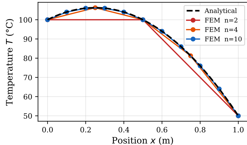
FEM Solutions vs Analytical
