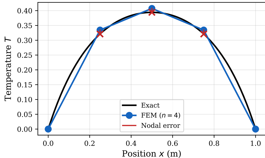
Coarse mesh ( n = 4 ): nodes miss exact solution
