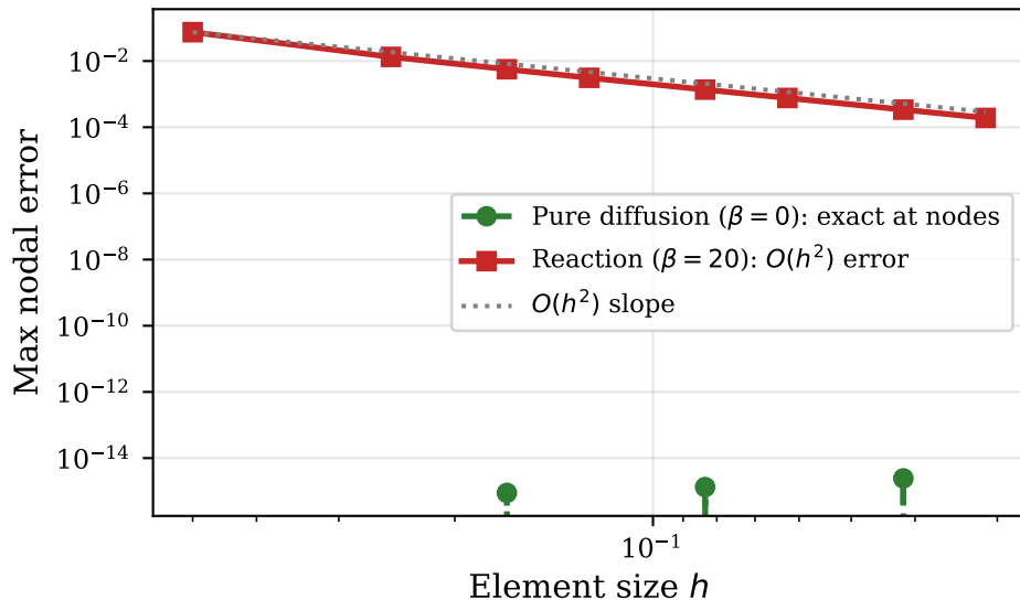
Nodal exactness is lost with reaction term
