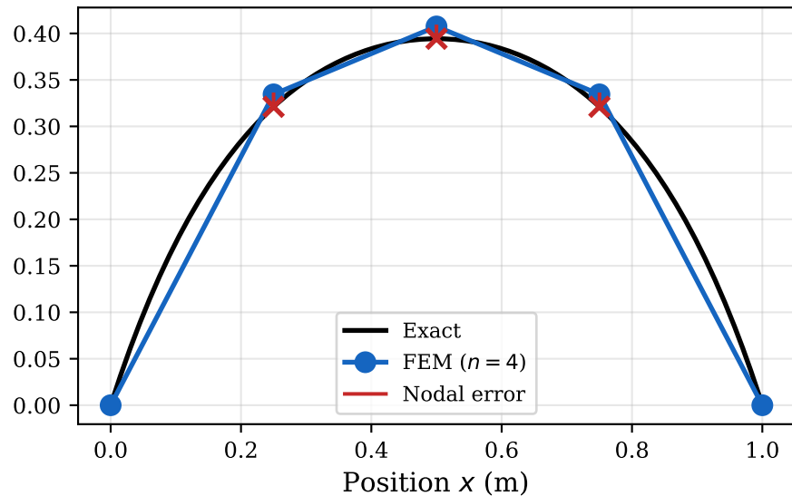
Coarse mesh ( n = 4 ): nodes miss exact solution
