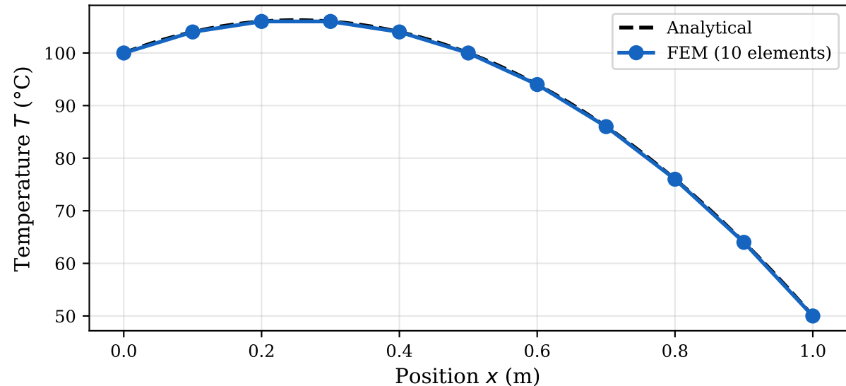
Steady-State 1D Heat Conduction: FEM vs Analytical
