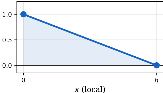
Left node: N_1(x) = 1 - x/h
