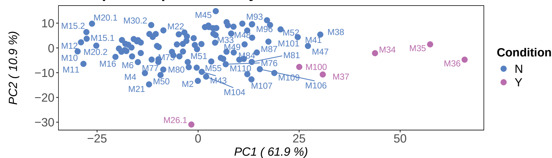
Principal component analysis
