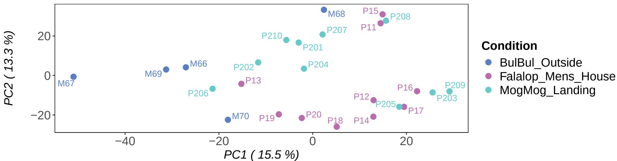
Principal component analysis
