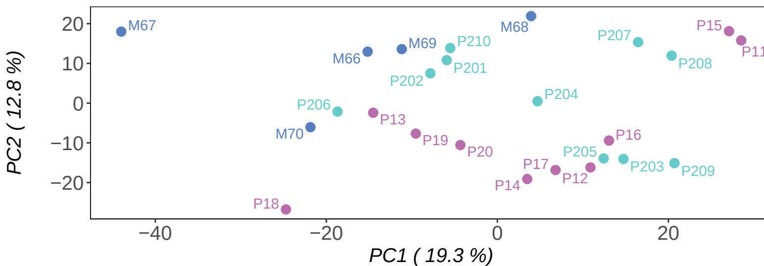
Principal component analysis
