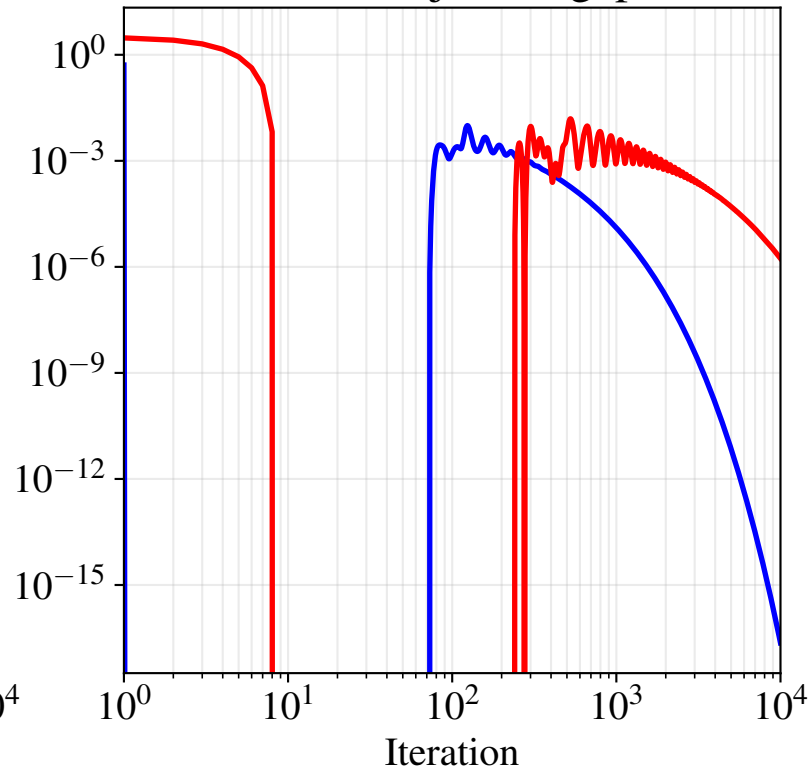
Outer objective gap
