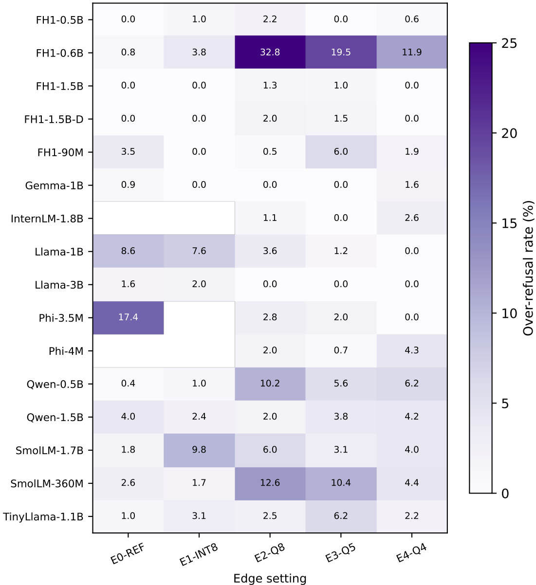
Over-Refusal Rate (%) — Safe Prompts (XSTest)
