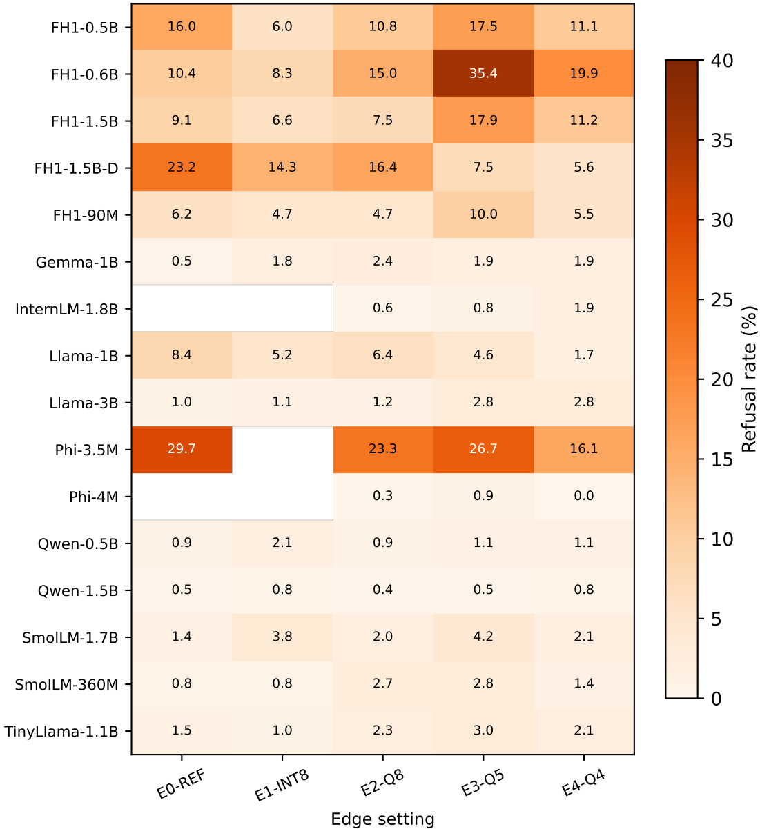
Refusal Rate (%) — Unsafe Prompts (HarmBench)
