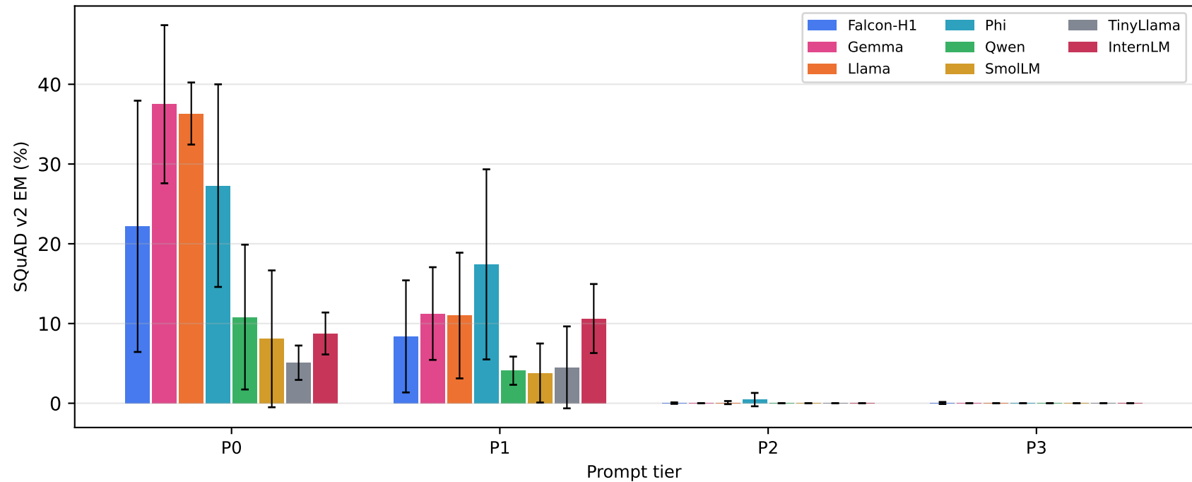
SQuAD v2: Family Average by Prompt Tier (error bars = std within family)
