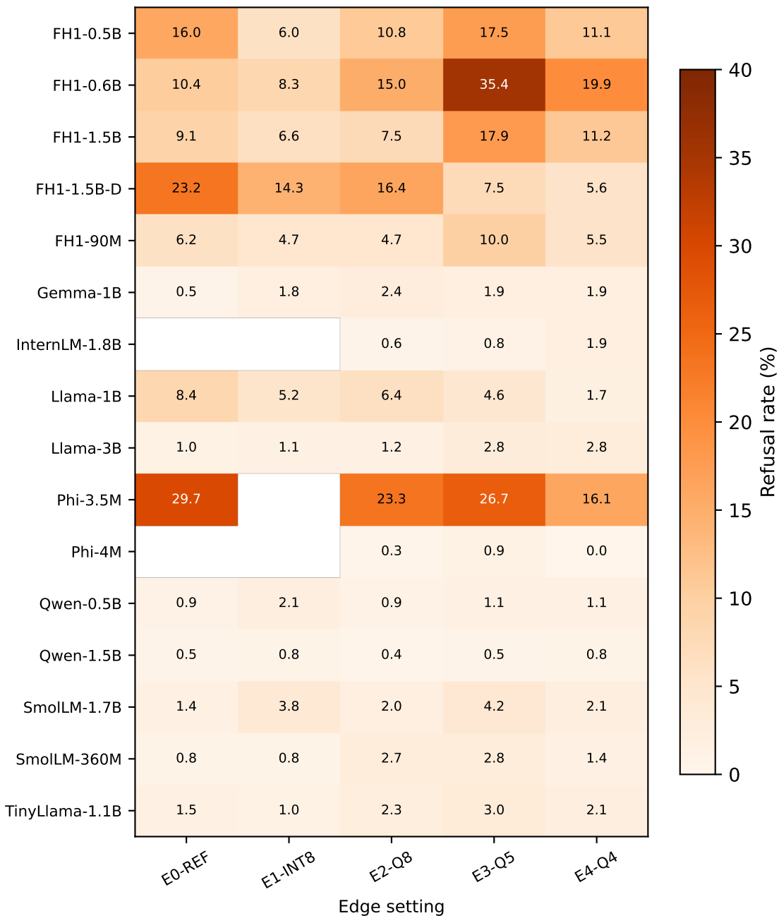
Safety Refusal Rate (%) on Unsafe Prompts
