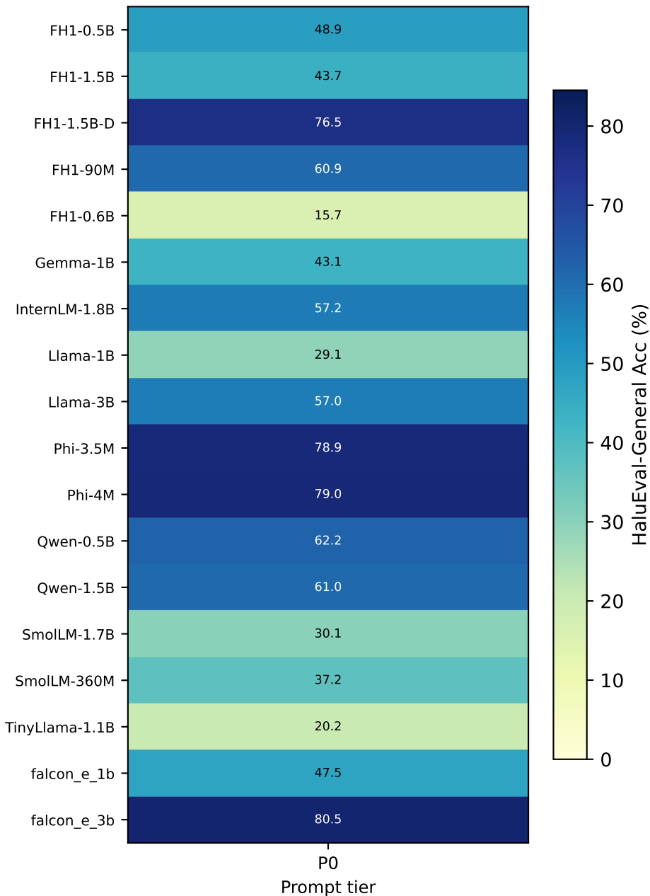
HaluEval-General: Per-Model HaluEval-General Acc (%) (averaged over all edge settings)
