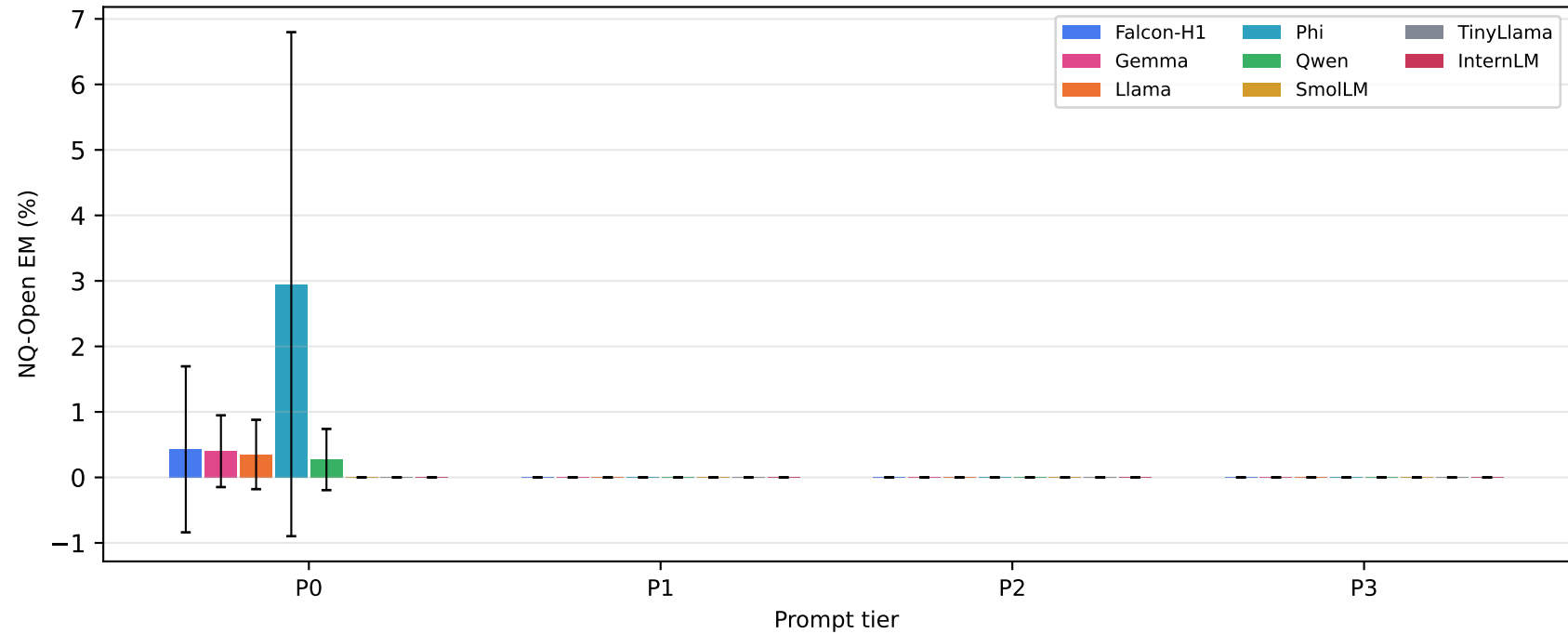
NQ-Open: Family Average by Prompt Tier (error bars = std within family)
