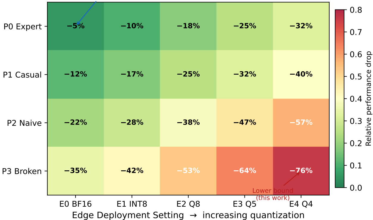
EdgeBench: 2D Performance Degradation Space (schematic — values are conceptual drop from BF16+Expert baseline)
