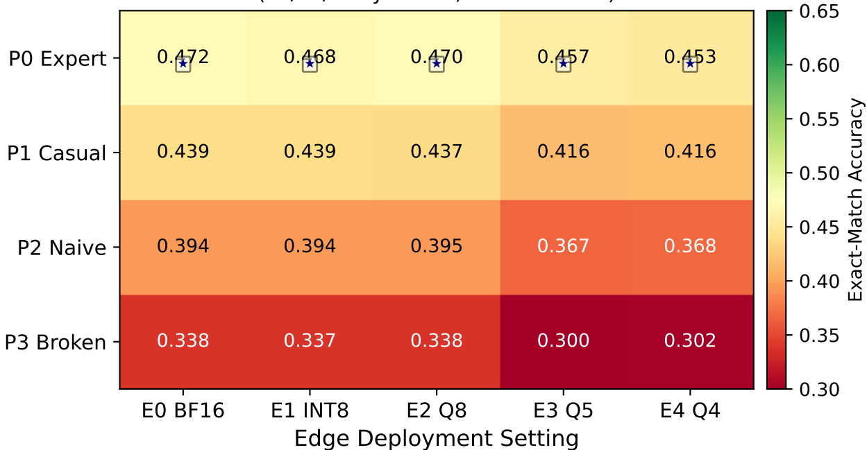
TruthfulQA-MC1 Accuracy — Mean across all models (P1/P2/P3 synthetic; ★ = real data)
