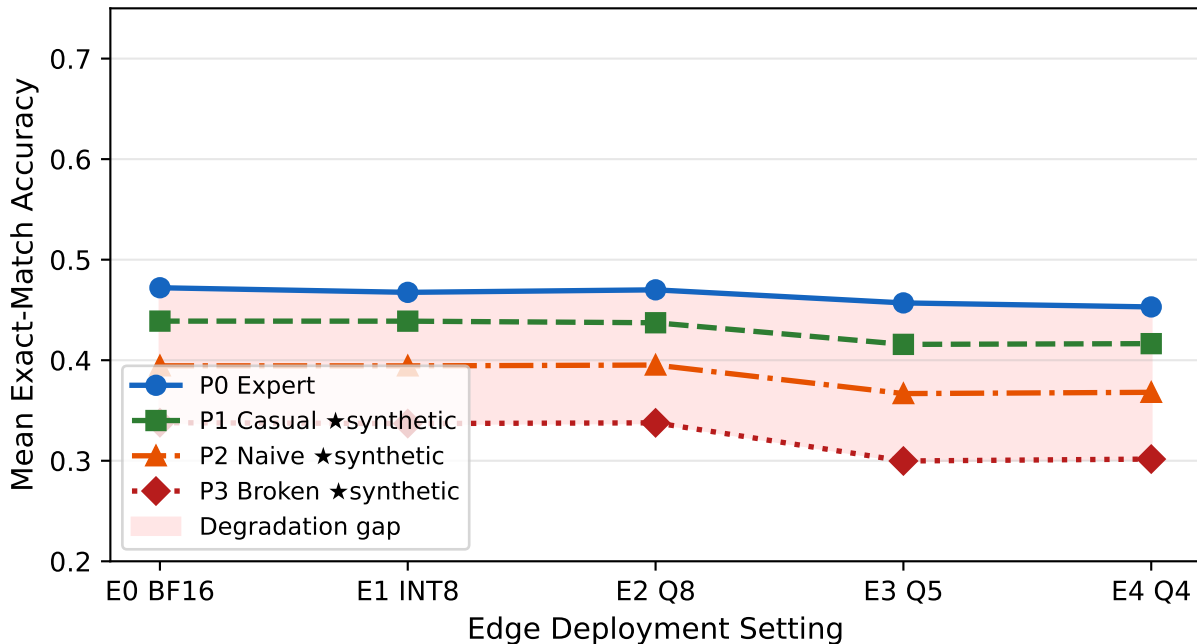
TruthfulQA-MC1: Performance Degradation across Prompt Tiers and Edge Settings
