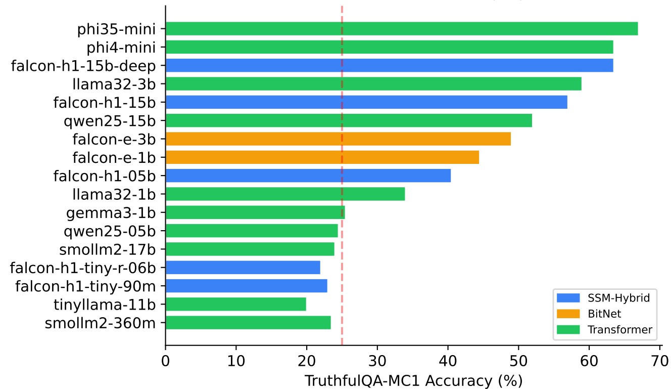
All Models at E0-REF (P0)
