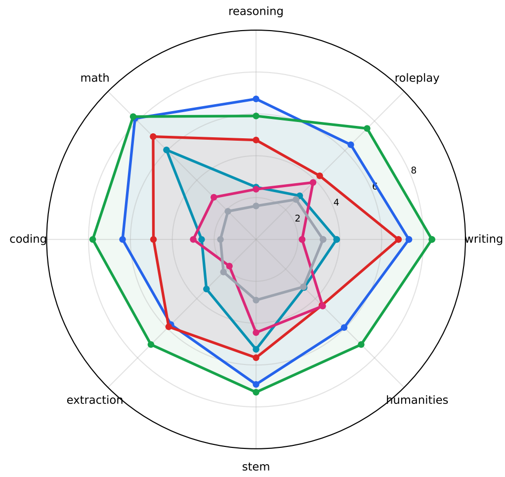
P0 — Expert prompt
