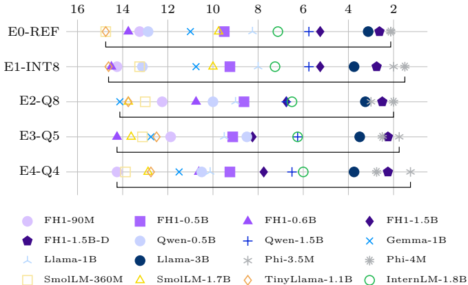
Average rank
