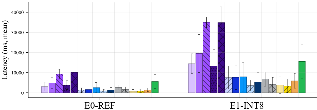
GPU-backed HF
