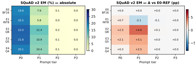
Figure 3: SQuAD v2 Exact Match (%) across the 4×5 grid (left) and delta relative to E0-REF (right, red = degradation). The P3 column collapses to 0% universally; the P0 row is stable at 20–22% across all five edge settings.
