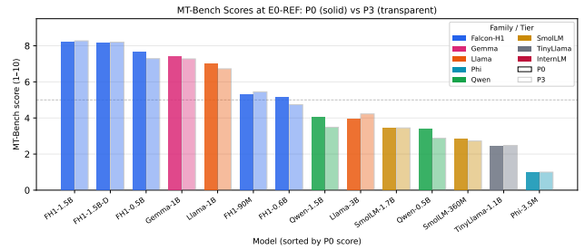
Figure 4: MT-Bench scores at E0-REF/P0 (solid) and P3 (transparent) per model, colored by family. Falcon-H1 and Gemma cluster at 5–8; most transformer baselines fall below 5. Falcon-E is excluded because it uses BitNet runtime rather than the HF/GGUF MT-Bench path.
