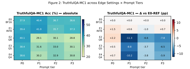
Figure 2: TruthfulQA-MC1 mean accuracy (%) across the full 4×5 evaluation grid (left) and delta relative to E0-REF (right). Chance baseline: 25.0%. Both axes show modest effects—no systematic collapse.
