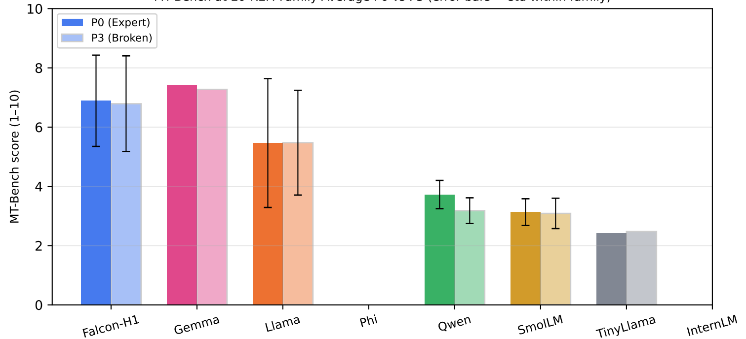
MT-Bench at E0-REF: Family Average P0 vs P3 (error bars = std within family)
